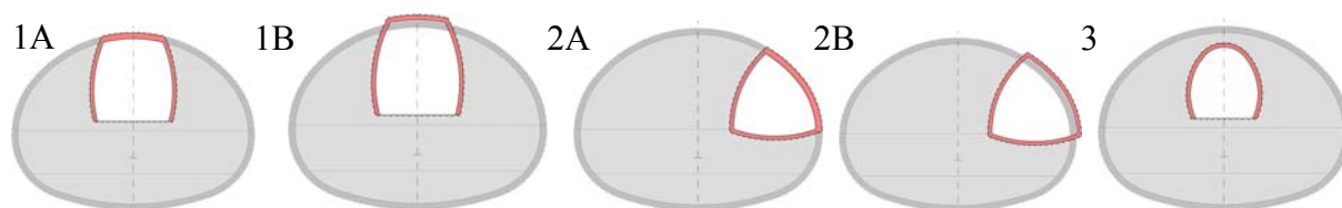
Fig. 4 Positions and geometries of pilot adits and their examples (1 - PCRR 513, PCRR 514; 2 – Královo Pole tunnel, Brno; 3 – Mrázovka, Královská Obora, Prackovice tunnels)
